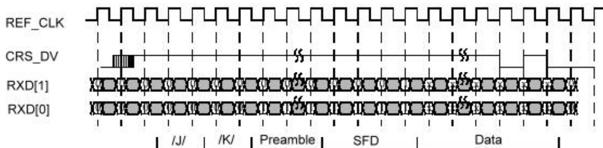
9.4.16 RMII Receive Timing Diagram
