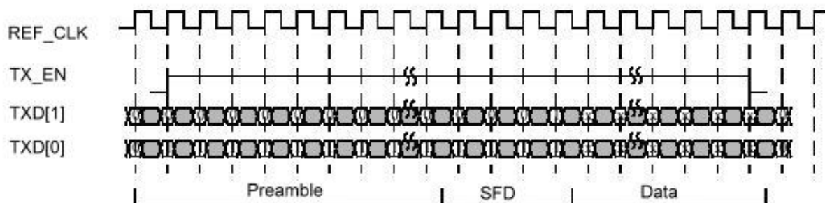
9.4.17 RMII Transmit Timing Diagram
