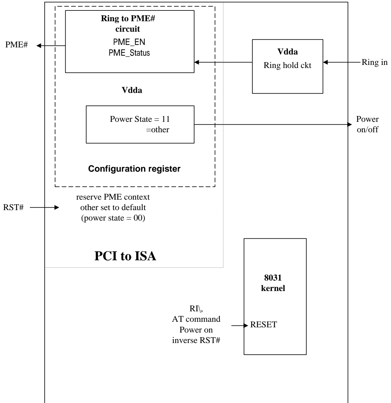
DM6588 PCI Power Configuration
