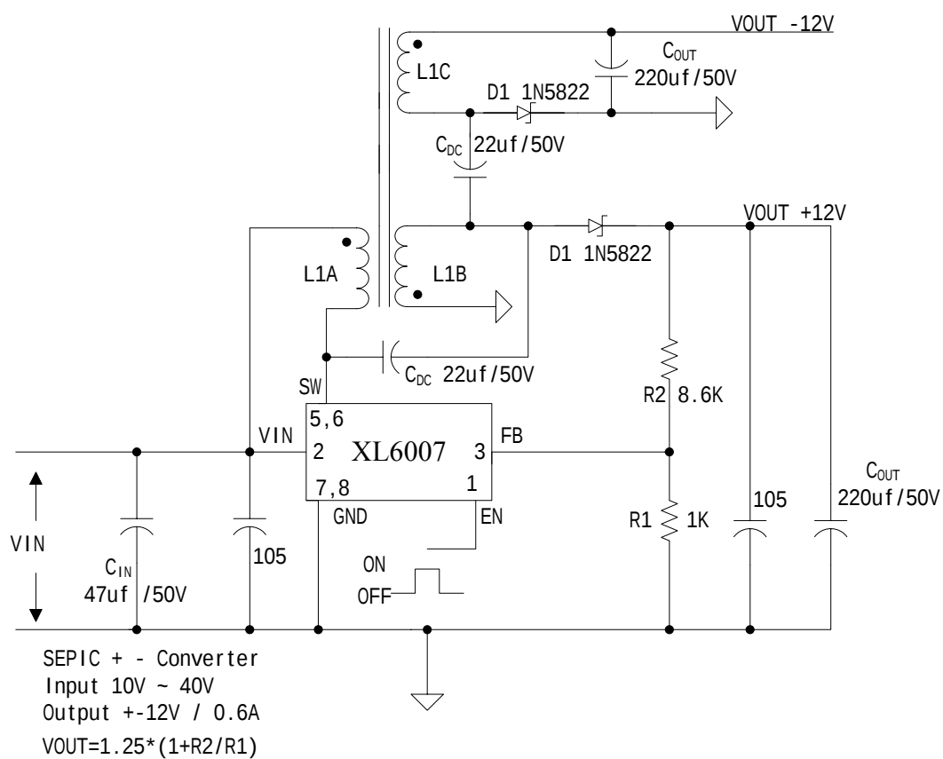
Figure8. XL6007 Typical System Application (SEPIC Inverting Converter)
