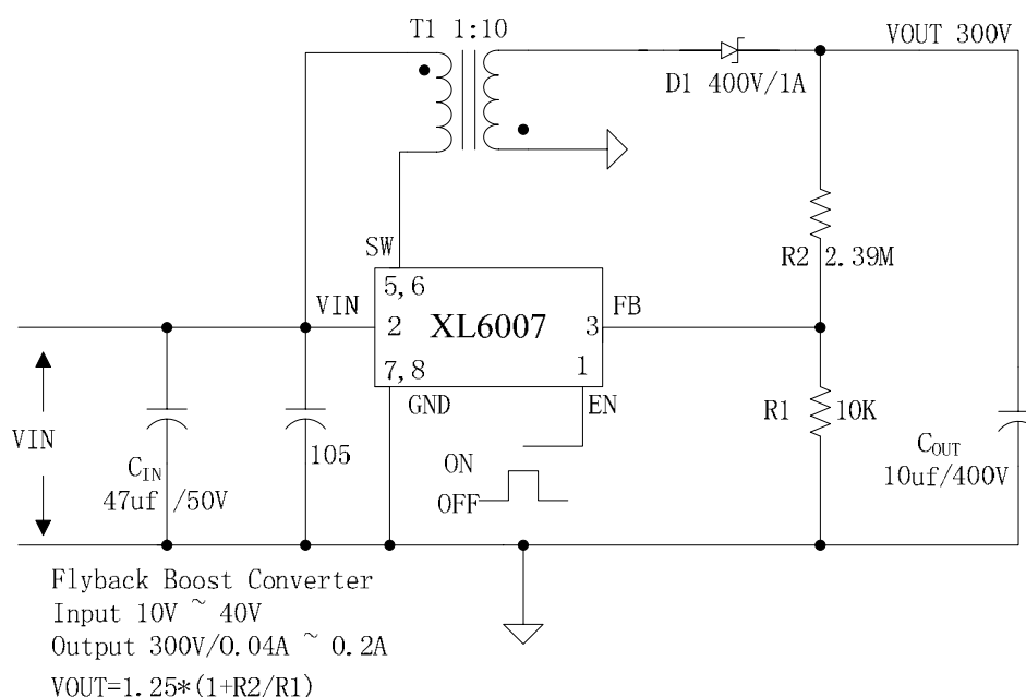
Figure7. XL6007 Typical System Application (Flyback Boost Converter)
