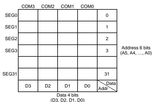
RAM mapping
