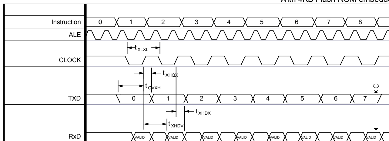
Figure5 UART waveform in Shift Register MODE
