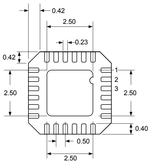
BOTTOM VIEW
