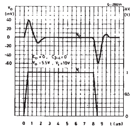
Figure 15. Voltage Transient Response.
