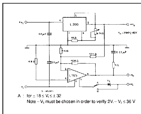
Figure 25. High Current Tracking Regulator.
