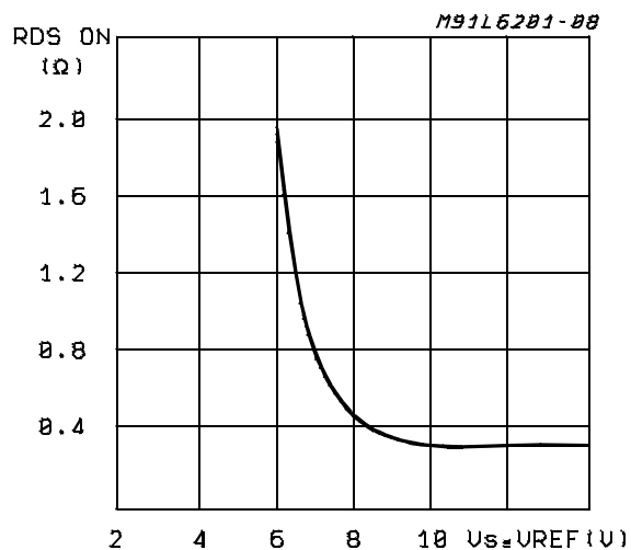
Figure 4: Typical R_{DS(ON)} vs. V_s \sim V_{ref}
