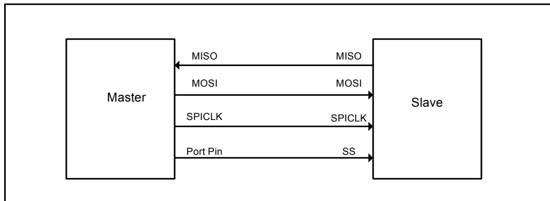
SPI single master single slave configurartion
