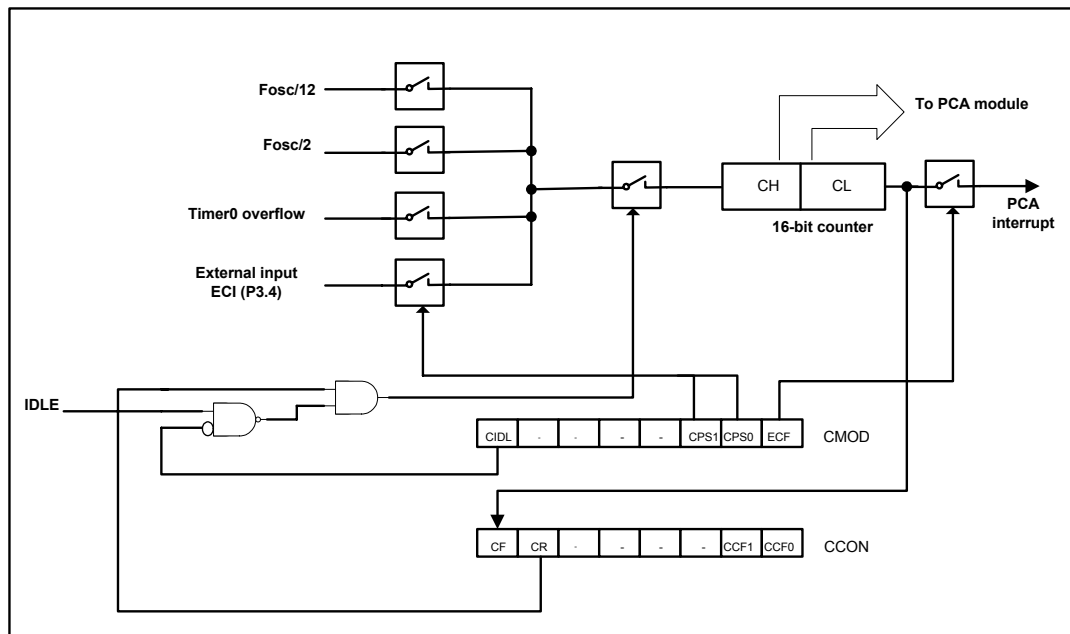
PCA Timer/Counter
